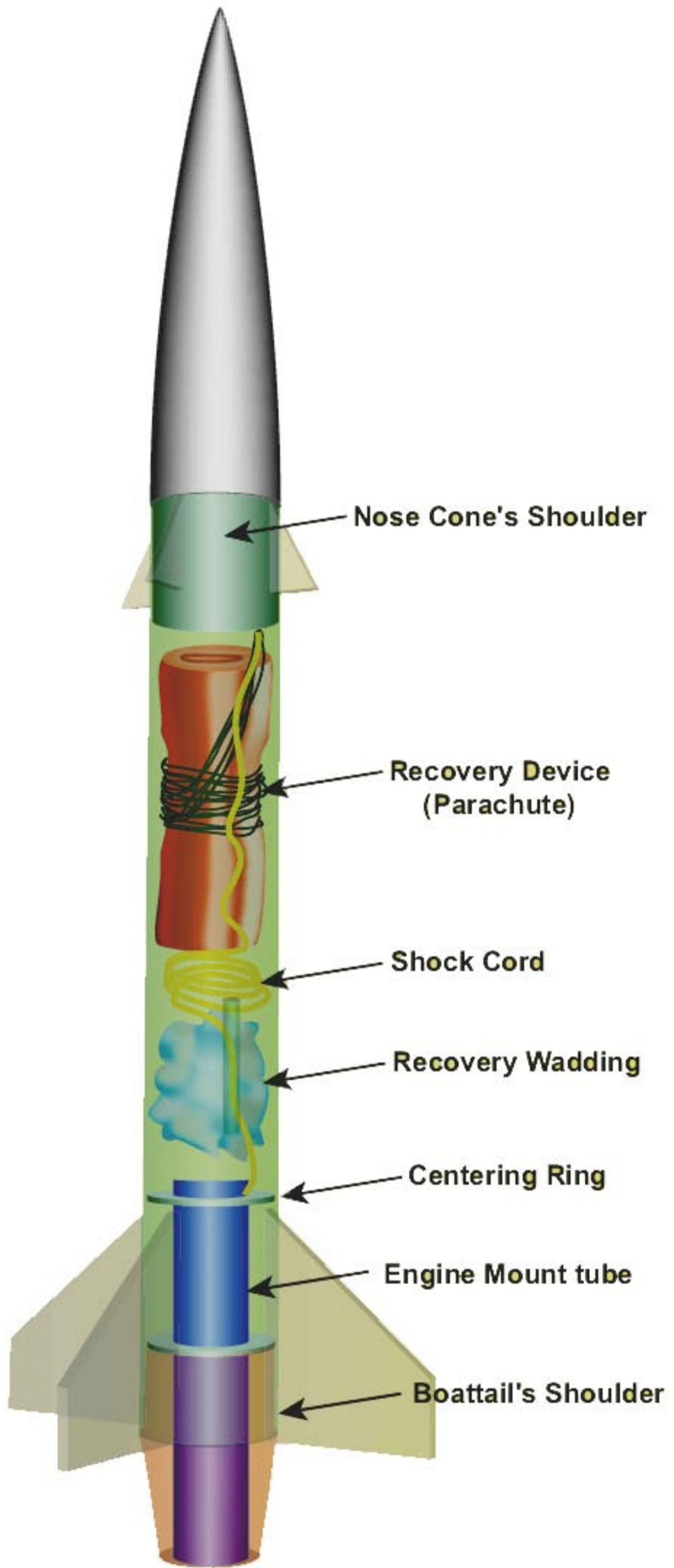
Internal Parts
